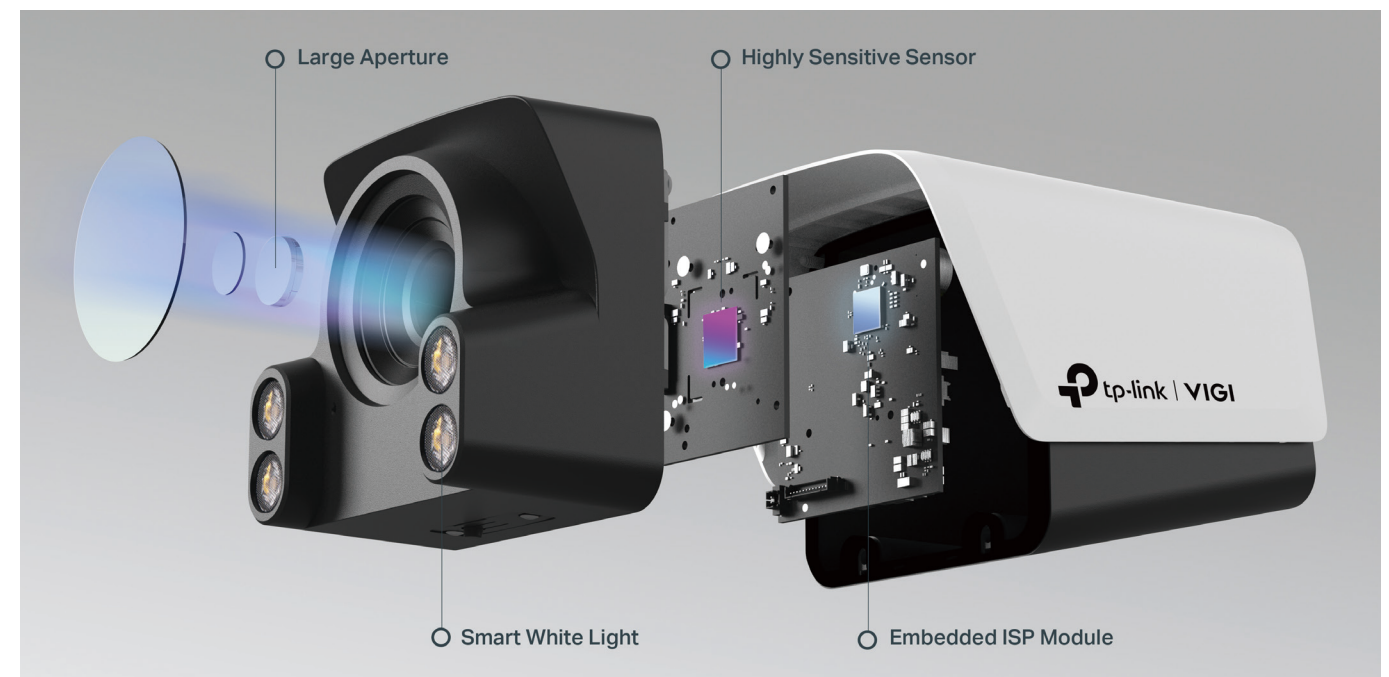
Naked Eyes
