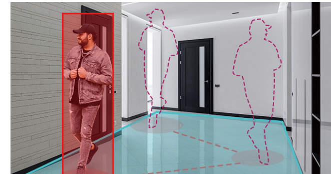
Loitering Detection
